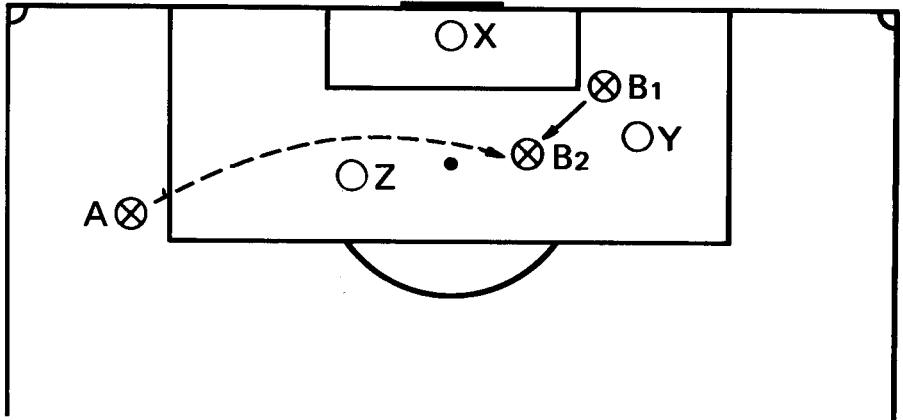
Diagram 5 – OFF-SIDE
