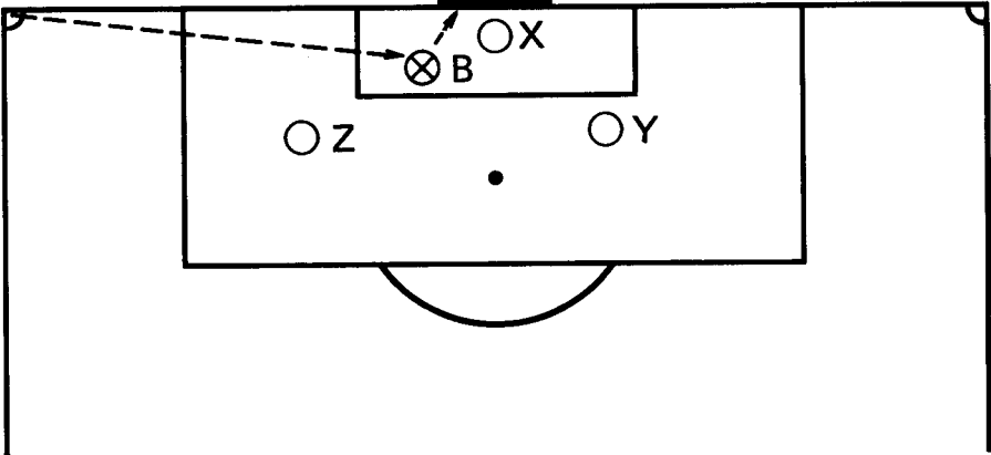
Diagram 15 – NOT OFF-SIDE
