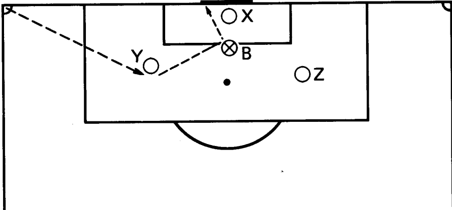
Diagram 16 – NOT OFF-SIDE
